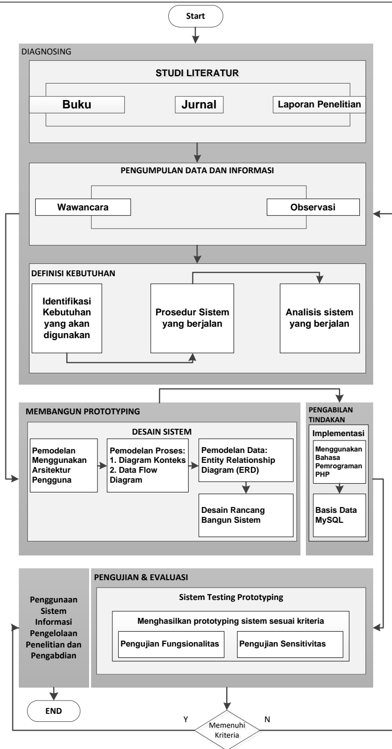
Gambar 1. Alur Penelitian
