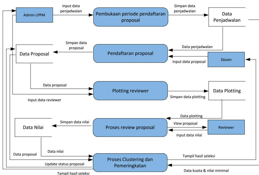
Gambar 4. Data Flow Diagram (DFD)
