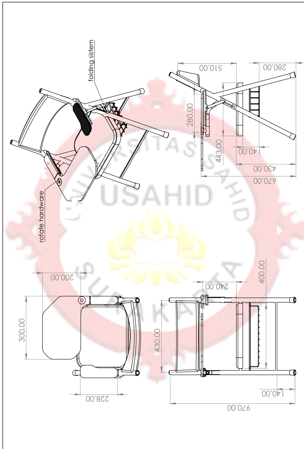
Lampiran 6. Gambar 2D Kursi Kuliah
